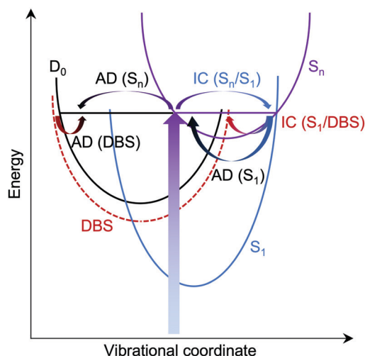
Fig. 8 Schematic potential energy diagram illustrating possible autodetachment (AD) and internal conversion (IC) processes, following photoexcitation of a resonance in the D_0 continuum, S_n . AD from S_1 is responsible for the continuum of low eKE electrons observed in phenolate-keto photoelectron spectra, AD from S_n is responsible for the broadening observed on the high eBE edge of the peak associated with direct detachment in phenolate-enol photoelectron spectra and S_1 /DBS IC followed by AD from the DBS is responsible for the low eKE peaks in the phenolate-enol and phenolate-enolate photoelectron spectra.
